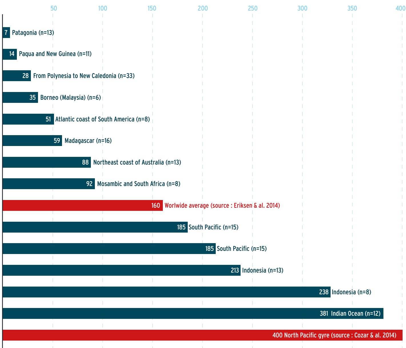
Average Micro + Mesoplastic concentration per region (g/km 2 )
